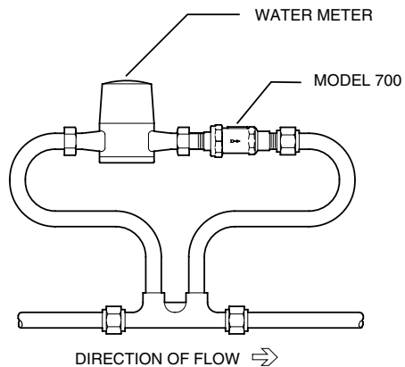
METER SETTER INSTALLATION
