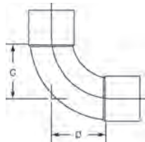
607-1 90° Elbow – Intermediate Radius C x C – Wrot
