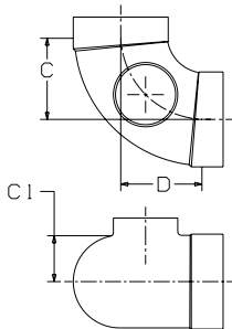
807-9 ⚠ DWV 90° Elbow w/Side Inlet C x C x C – Cast
