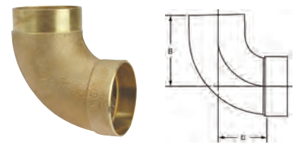
807-2 ⚠️ DWV 90° Fitting Elbow Ftg x C – Cast
