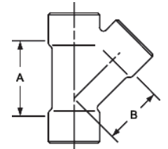
749 ⚠ 45° Y C x C x C – Cast
