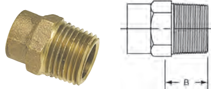
704 ⚠ Adapter C x M – Cast
