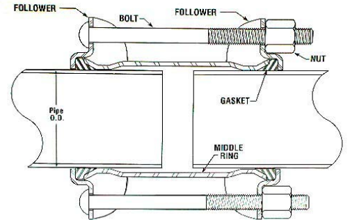
Anatomy of a Style 38 Dresser Coupling
