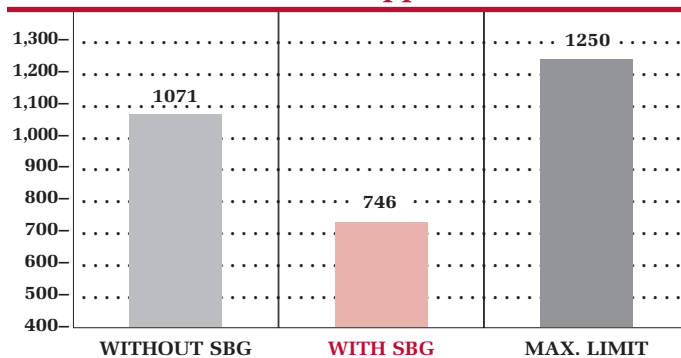
SO2 ppm
