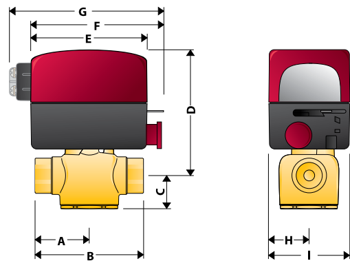
Dimensions for actuators with or without auxiliary switch.
