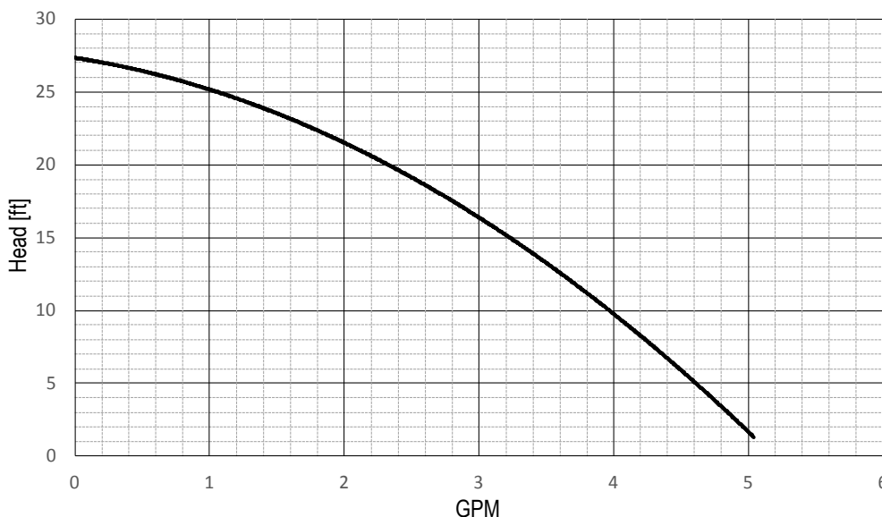
CB199-DV / CB180-DV Pump Performance ( with internal pressure drop)
