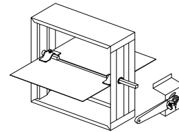
422-XS MANUAL VOLUME DAMPER
