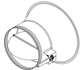
3200-DS CONICAL SPIN-IN with \frac{3}{8} " SOLID ROD AXIS & 2" STANDOFF (14" - 20")
