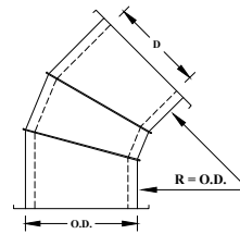
DW6121 45° ELBOW 3 Piece Gorelock
