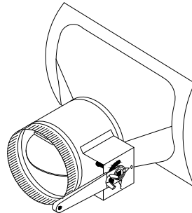
3305-DS2 TAKEOFF with \frac{3}{8} " SOLID ROD AXIS & 2" STANDOFF (6" - 12")
