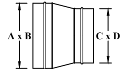
FO6265 REDUCER
