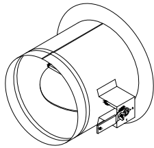
3710-DS TAKEOFF with 2" DAMPER HANDLE STANDOFF (4" - 12")
