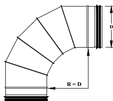
E6111 90° ELBOW 14" - 36" 5 Piece Gorelock
