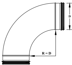
E6111 90° ELBOW 4" - 12" Die Stamped
