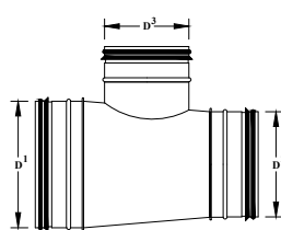
E6271R REDUCING TEE
