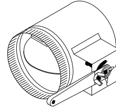
175-XS2 DAMPER SLEEVE with \frac{3}{8} " SOLID ROD AXIS & 2" STANDOFF (4" - 20")
