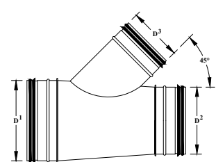
E6276R REDUCING LATERAL
