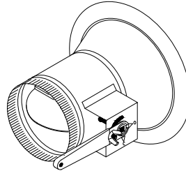
3210-DS2 CONICAL with \frac{3}{8} " SOLID ROD AXIS & 2" STANDOFF (4" - 12")
