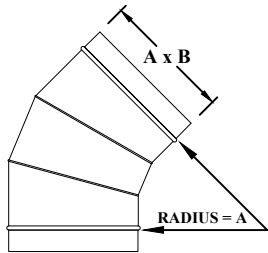
FO6121 HARD BEND 45° ELBOW
