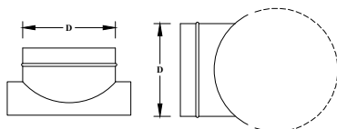
SP6307 90° SADDLE TAP
