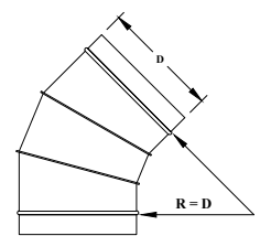
SP6121 45° ELBOW 14" - 48" 3 Piece Gorelock
