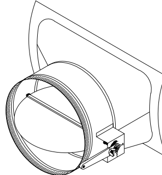
3305-DS TAKEOFF with \frac{3}{8} " SOLID ROD AXIS & 2" STANDOFF (14" - 20")
