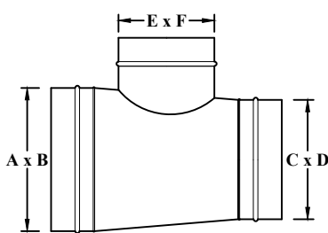
FO6271R REDUCING 90° TEE
