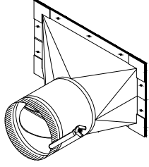
3300-D 45° TAKEOFF with DAMPER
