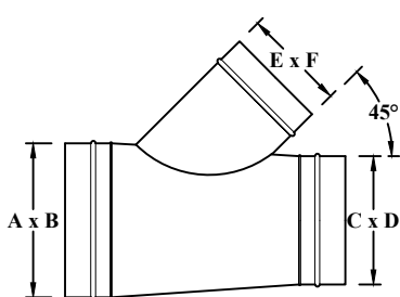
FO6276R REDUCING 45° LATERAL
