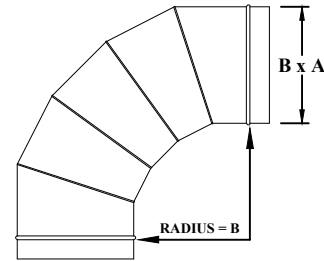
FO6112 EASY BEND 90° ELBOW
