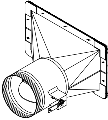
3300-DS 45° TAKEOFF with 2" DAMPER HANDLE STANDOFF (4" - 12")
