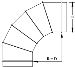
SP6111 90° ELBOW 14" - 48" 5 Piece Gorelock
