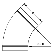
SP6121 45° ELBOW 4" - 12" Die Stamped
