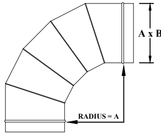
FO6111 HARD BEND 90° ELBOW
