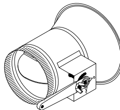
3200-DS2 CONICAL SPIN-IN with \frac{3}{8} " SOLID ROD AXIS & 2" STANDOFF (4" - 12")
