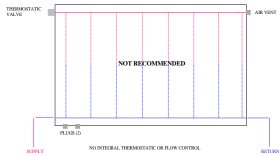
PENSOTTI PANEL RADIATORS - ALTERNATE PIPING ARRANGEMENT 3
