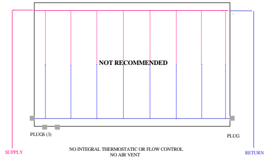
PENSOTTI PANEL RADIATORS - ALTERNATE PIPING ARRANGEMENT 4
