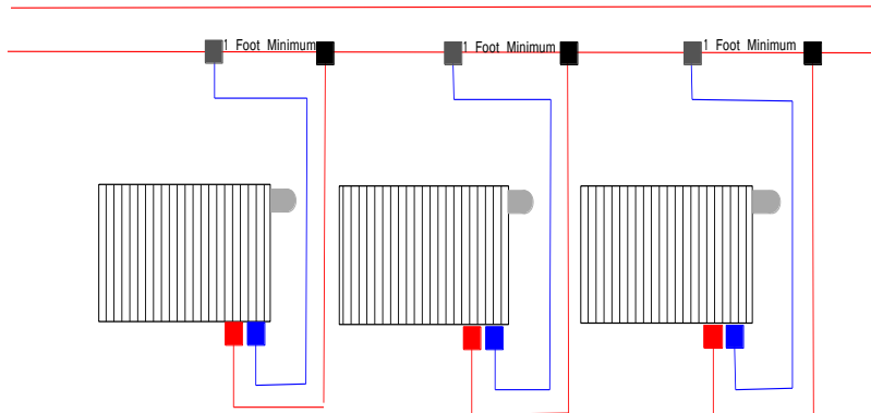
Downflow Monoflo w/ Thermostatic Operators*
