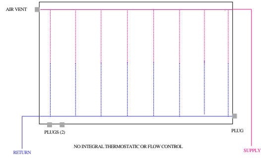
PENSOTTI PANEL RADIATORS - ALTERNATE PIPING ARRANGEMENT 2
