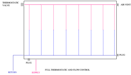
PENSOTTI PANEL RADIATORS - ALTERNATE PIPING ARRANGEMENT 5
