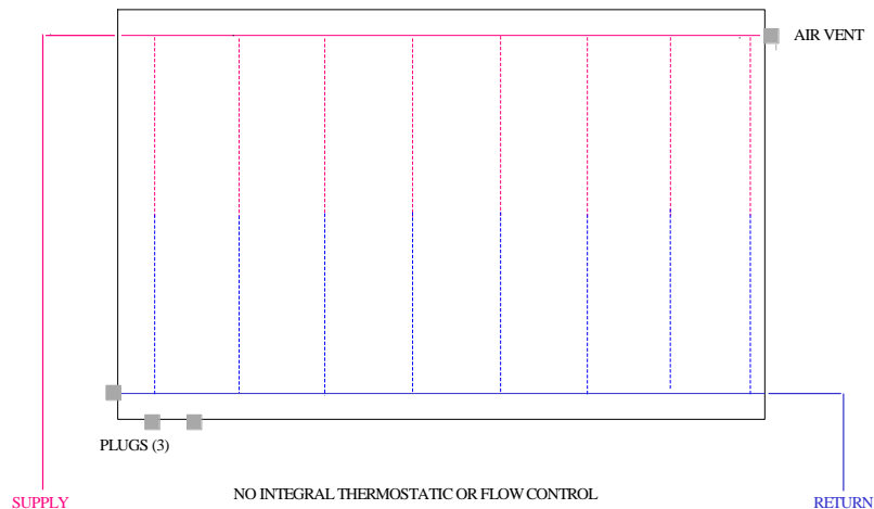
PENSOTTI PANEL RADIATORS - ALTERNATE PIPING ARRANGMENT 1
