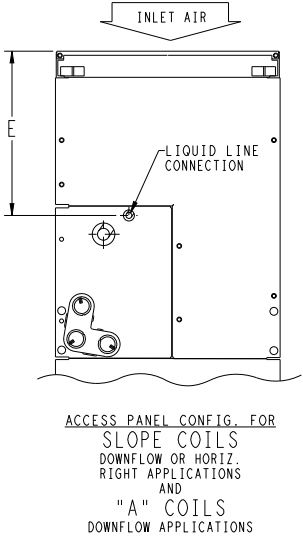
Fig. 3 – FHMA5 - Metric (sheet 1)
