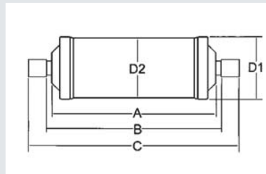
Solder Connection
