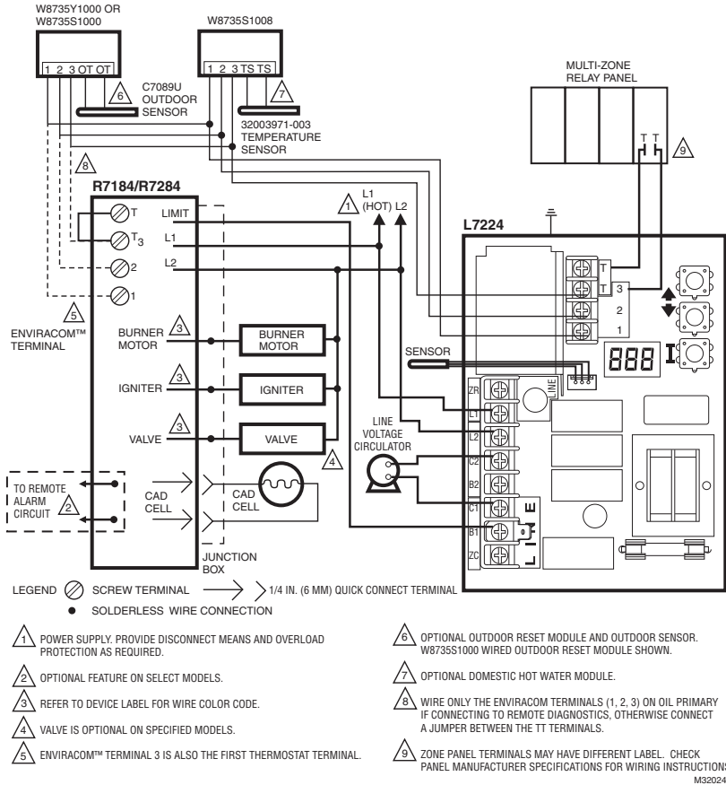
Fig. 11. L7224U multizone system with Outdoor Reset and Domestic Hot Water Modules (indirect tank applications).
