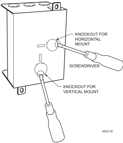
Fig. 2. Removing horizontal or vertical mounting knockout.
