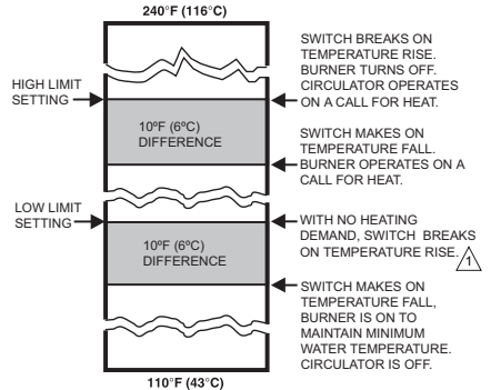
△ WHEN WATER REACHES LOW LIMIT SETTING, THE BURNER SHUTS OFF OR THE CIRCULATOR PUMP STARTS (WHEN CALLING FOR HEAT).
