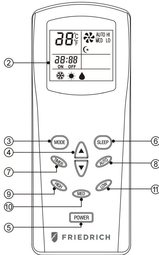
Front view
