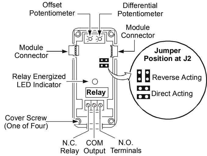
Figure 4: Interior View and Typical Wiring of the S352A Stage Module
