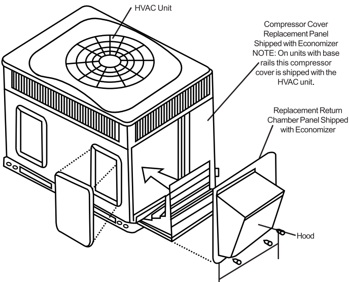
Vertical Economizer
