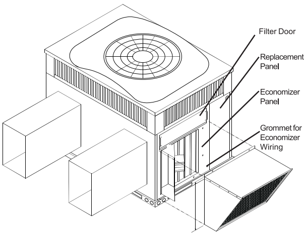
Horizontal Economizer
