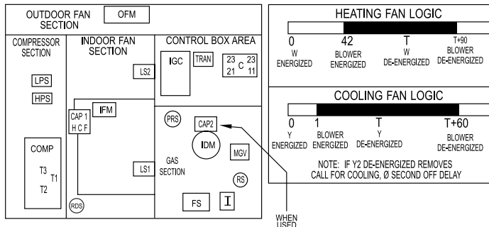
10 UNIT COMPONENT ARRANGEMENT
